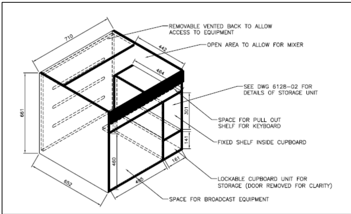
3d View (minus Lid and Mixer Top)
